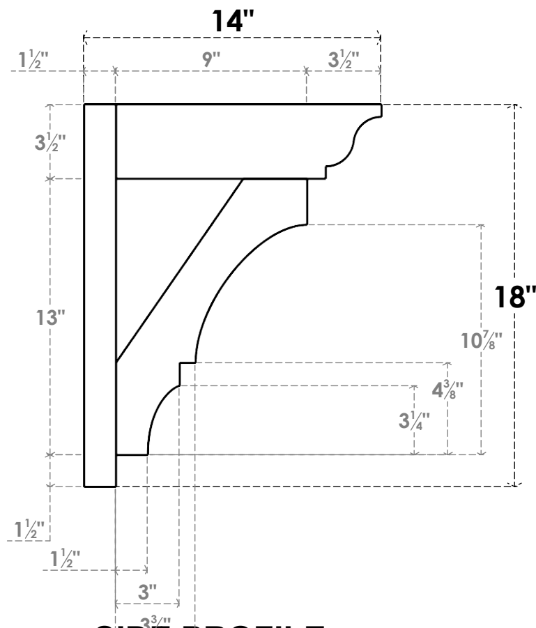
SIDE PROFILE
